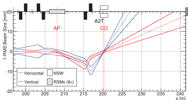
Figure 4: A2T schematic layout and RMS beam envelopes inside (courtesy of H. D. Thomsen).
