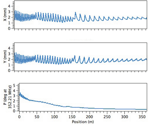
Figure 2: Beam rms sizes in three planes, Top: X , Middle: Y , Bottom: \phi at 352.21 MHz.
